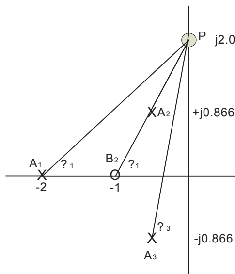
Figure 3.6 Graphical evaluation of a frequency response from the zero-pole plot.
