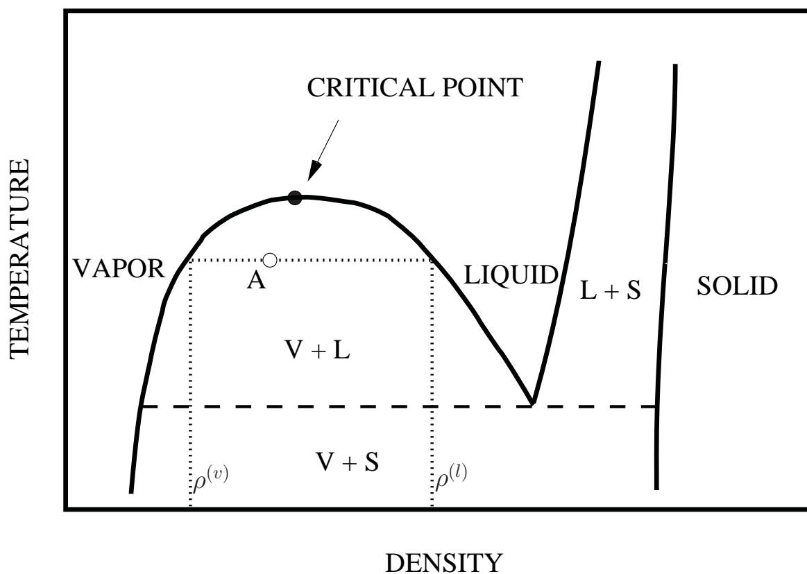
Figure 2.2: Temperature-density diagram for a general pure substance.
